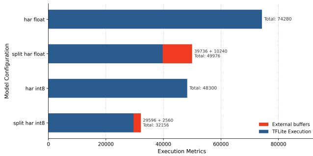
Figure 8: Graph of peak RAM usage of the HAR models
