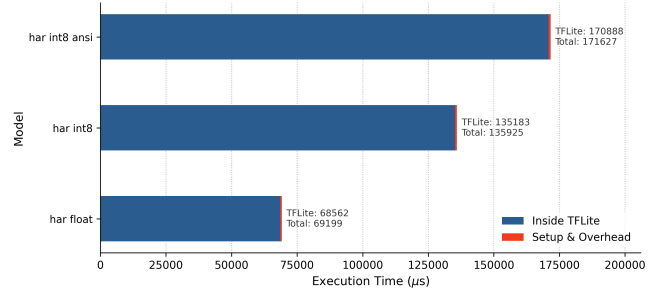
Figure 5: Graph of the latency of the HAR models
