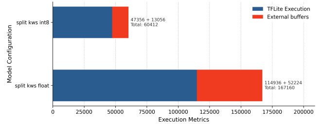
Figure 9: Graph of peak RAM usage of the KWS models
