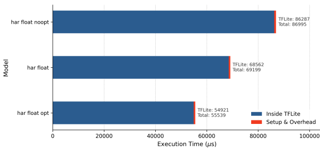
Figure 4: Comparison of different amounts of exponentiation being eliminated from the float HAR model
