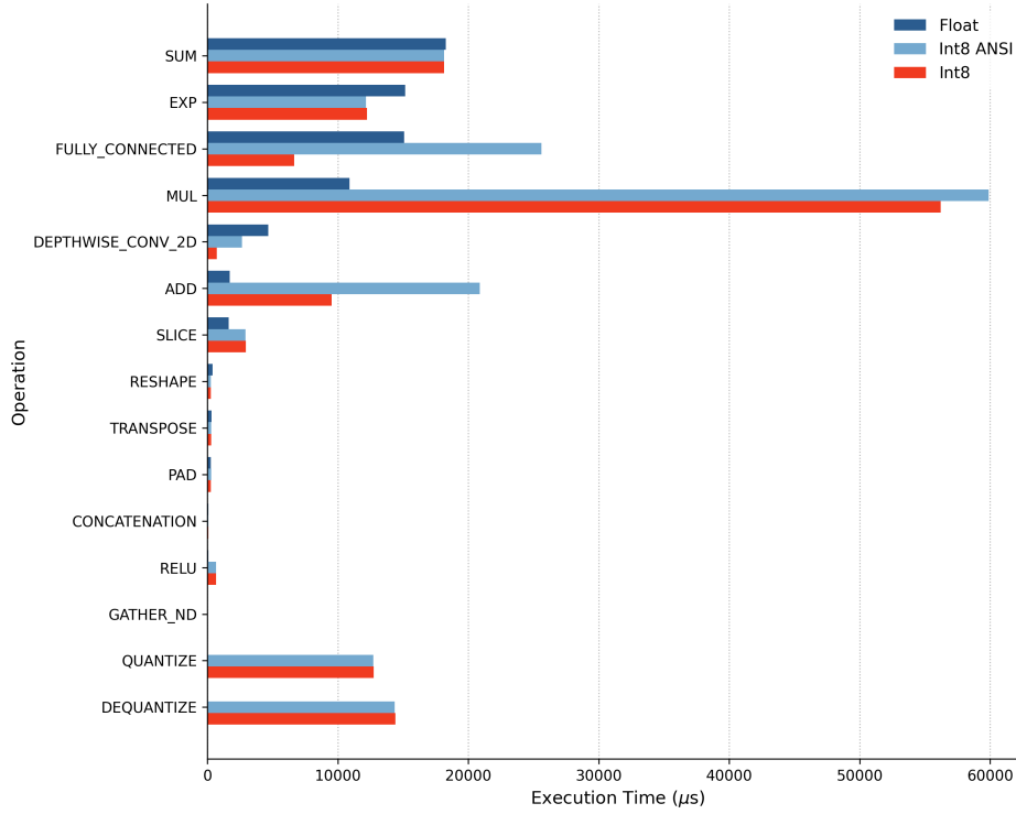
Figure 7: Comparison of operation impacts on latency of the Float, INT8 ANSI, and INT8 HAR models
