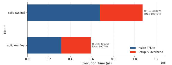
(b) Latency comparison between KWS float32 and int8 models
