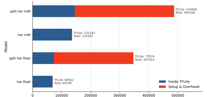
(a) Latency comparison between the HAR models
